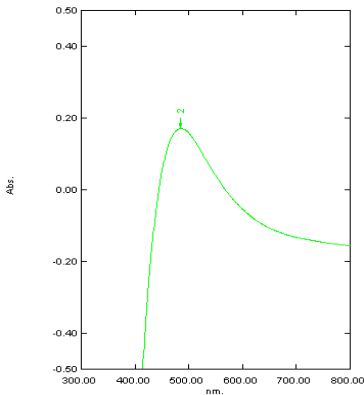
Figure-3 The UV spectrum of Oryza sativa silver nanoparticles recorded at room temperature
