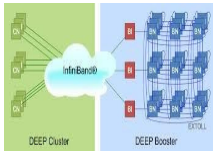
Figure-5 Deep cluster-booster architecture
