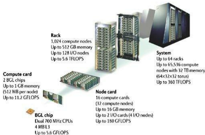
Figure-4 Blue brain Storage hierarchy
